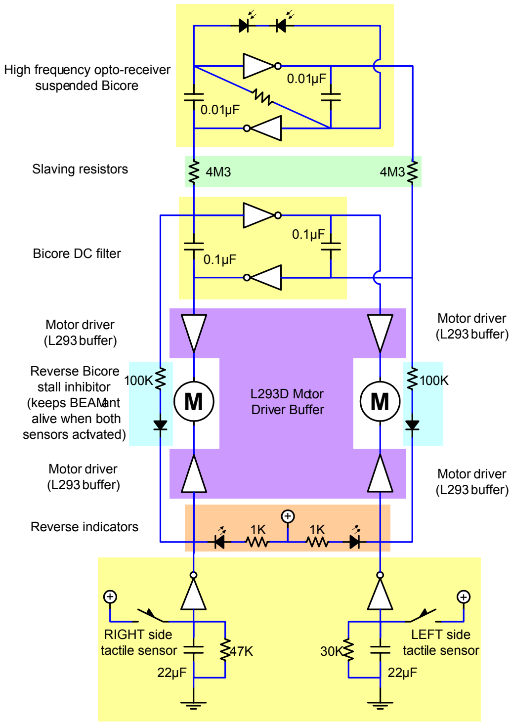
Motor polarity changing circuit (backup with timeout RC circuit)
